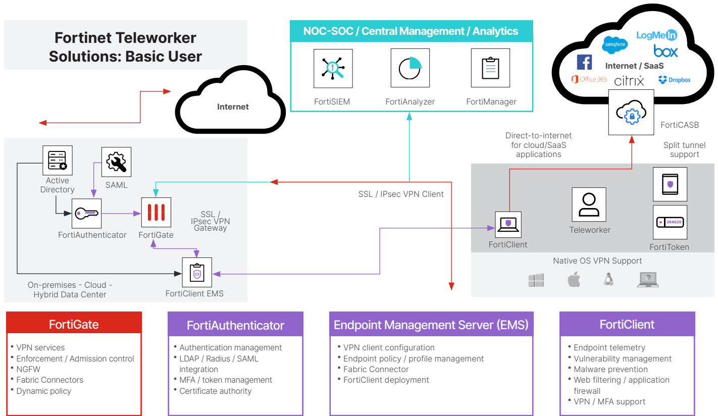
Figure 1: Notional Fortinet solution deployment for basic telemworker.
